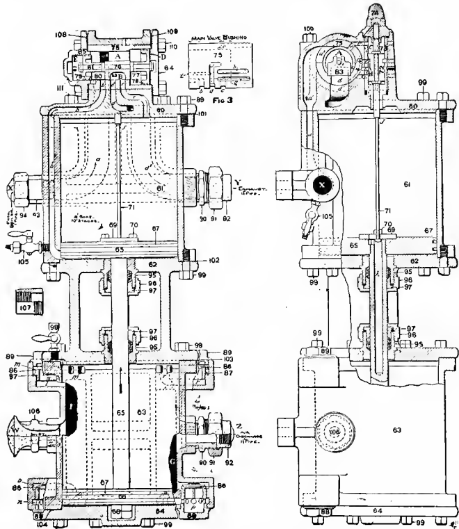
Fig. 1691. Longitudinal Section.
